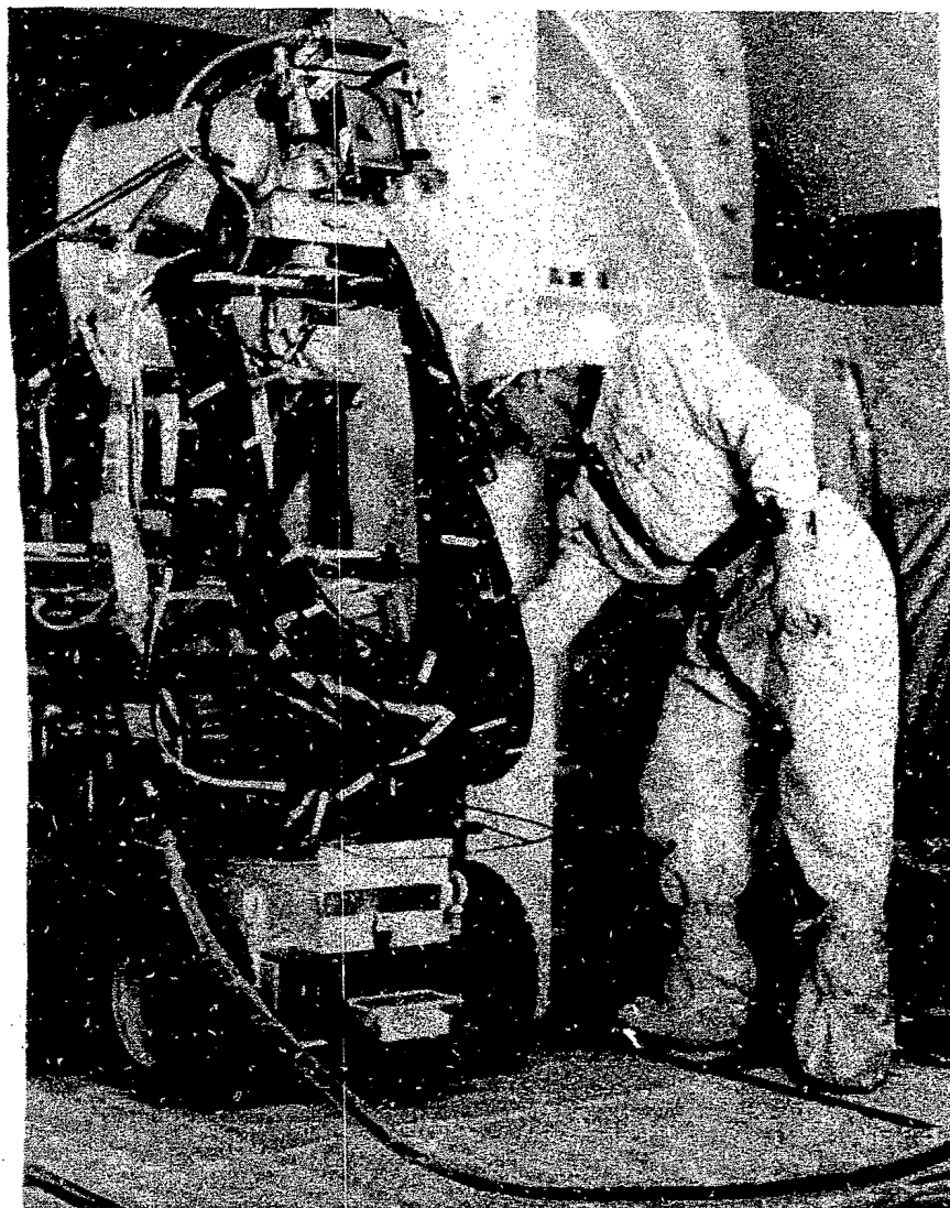
Figure 10. This 6-ft-tall, remote-controlled vehicle used radiation instruments and three television cameras to inspect the TMI-2 basement.
